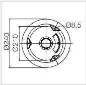
base dimensions
