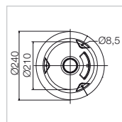
base dimensions
