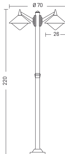
Pole | 2 lights cod. P2
