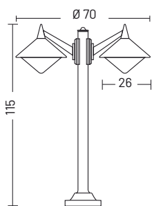
bollard cod. P2.12
