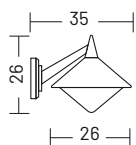
downwards wall lamp cod. 01
