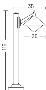
bollard cod. P1.12
